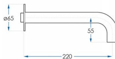
SPIN In Wall Basin/Bath Spout SP090 -200-CH / SP090 -200-MB / SP090 -200-BB / SP090 -200-BN SP090 -220-CH / SP090 -220-MB / SP090 -220-BB / SP090 -220-BN
