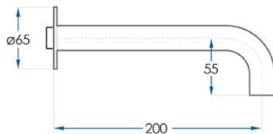
SPIN In Wall Basin/Bath Spout SP090 -200-CH / SP090 -200-MB / SP090 -200-BB / SP090 -200-BN SP090 -220-CH / SP090 -220-MB / SP090 -220-BB / SP090 -220-BN
