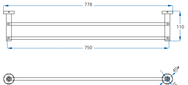
SPIN Double Towel Rail 750mm SP48-750-CH / SP48-750-MB / SP48-750-BB / SP48-750-BN
