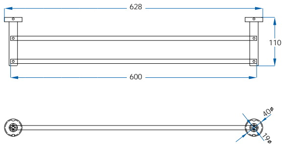
SPIN Double Towel Rail 600mm SP48-600-CH / SP48-600-MB / SP48-600-BB / SP48-600-BN
