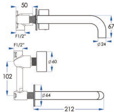
SPIN/MESH In Wall Progressive Mixer & 200mm Spout Set * WELS 5 Star, 6 ltr/min SP136-200-CH / SP136-200-MB / SP136-200-BB / SP136-200-BN SPM136-200-CH / SPM136-200-MB / SPM136-200-BB / SPM136-200-BN
