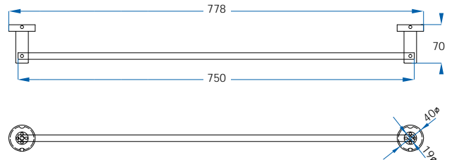
SPIN Single Towel Rail 750mm SP24-750-CH / SP24-750-MB / SP24-750-BB / SP24-750-BN
