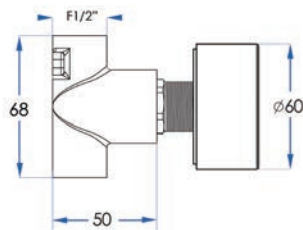
SPIN/MESH In Wall Progressive Mixer Set SP176-CH / SP176-MB / SP176-BB / SP176-BN SPM176-CH / SPM176-MB / SPM176-BB / SPM176-BN
