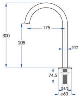
SPIN Basin/Bath Hob Spout WELS 6 Star, 4.5 ltr/min SP115-CH / SP115-MB / SP115-BB / SP115-BN
